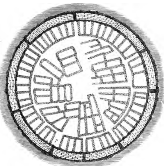
376. Ismantorps borg, plan.
